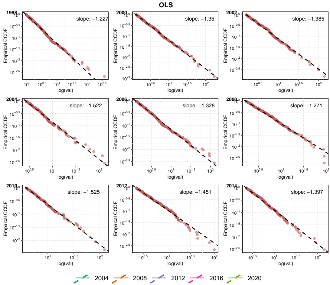
Figure 12. Wealth: log-log plots and Pareto tail coefficient estimates.
