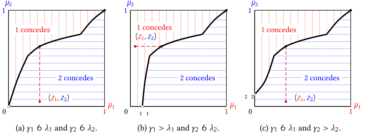
Figure 4: Reputation coevolution curves and initial concessions in games with two-sided ultimatum and single demand types when \gamma_i < \lambda_i for some i = 1, 2 .
