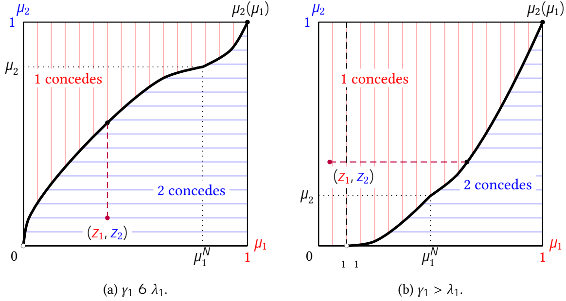
Figure 1: Reputation coevolution and initial concession in games with one-sided ultimatum. The solid line in each panel depicts the reputation coevolution curve \mu_2(\mu_1) . Player 1 concedes with a positive probability at time 0 when (z_1, z_2) is strictly to the left of the curve, player 2 concedes with a positive probability at time 0 when (z_1, z_2) is strictly to the right of the curve, and neither player concedes with a positive probability at time 0 when (z_1, z_2) is on the curve. The probability of initial concession ensures that the posterior reputation vector after initial concession lies on the curve. The reputations coevolve to (1, 1) according to the curve. When player 2's reputation reaches \mu_2 , player 1 stops challenging, and player 1's reputation \mu_1^N at the time is derived from the reputation coevolution curve.
