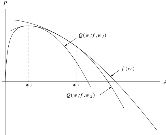
Figure 4: Quadratic approximations.
