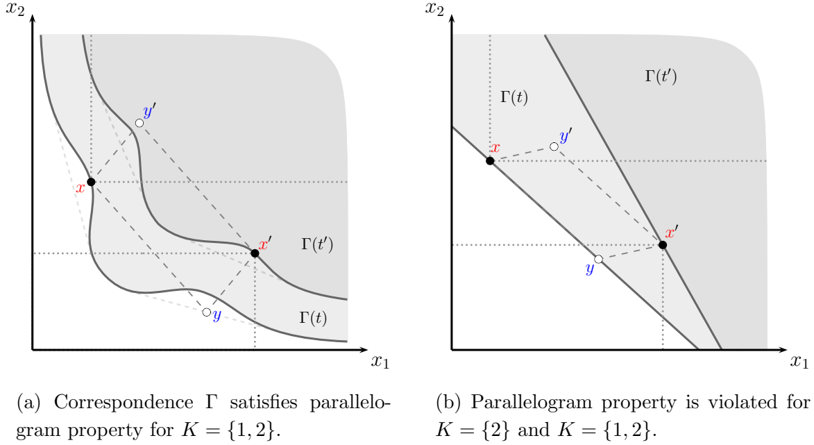
Figure 1: Geometric interpretation of parallelogram property.
