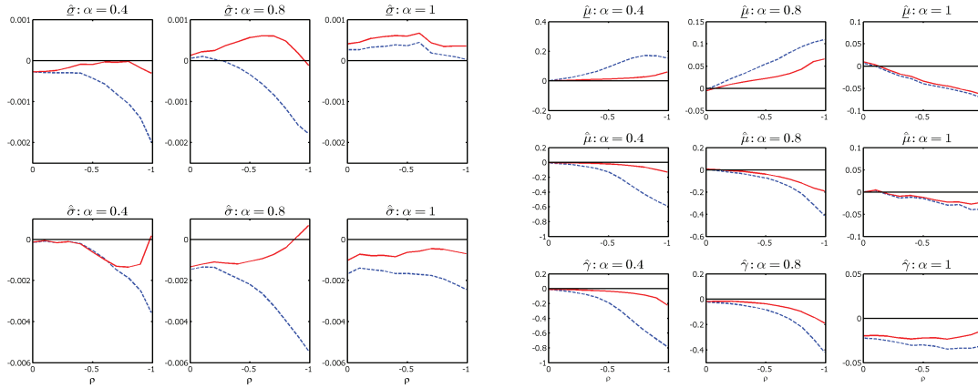
Figure 3: Endogeneity Bias
